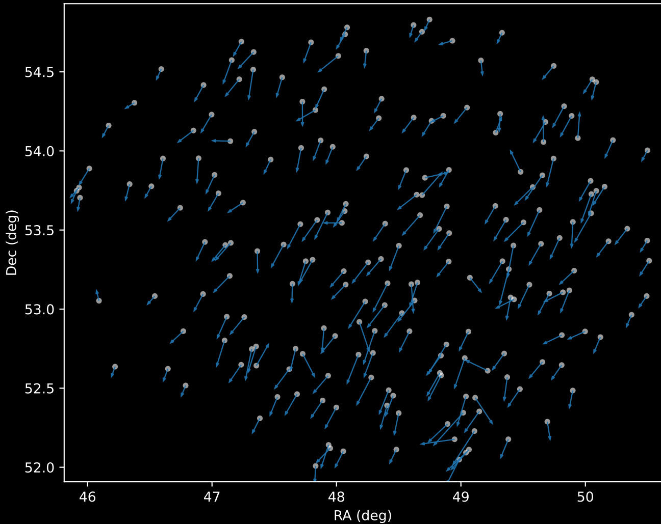
APOGEE DR17 Cluster 0 Proper Motion Vectors (n=202)
