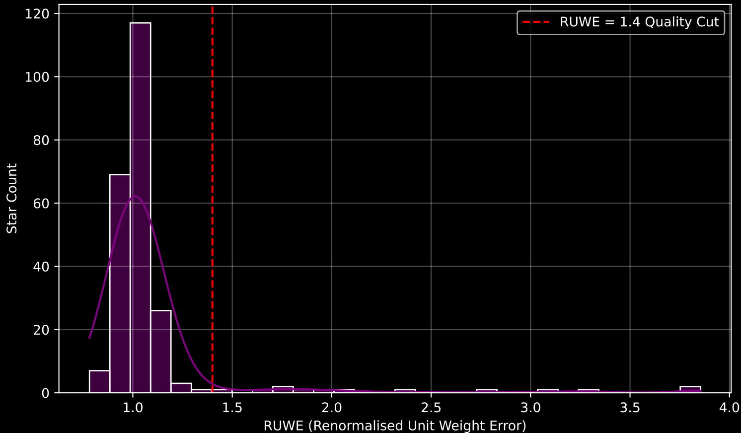
GAPOGEE DR17 Field [090+08] RUWE Distribution (n= 236)
