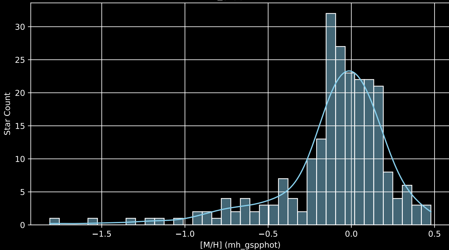
APOGEE DR17 Field: [090+08 [M/H] (mh_gspphot) (n= 236)
