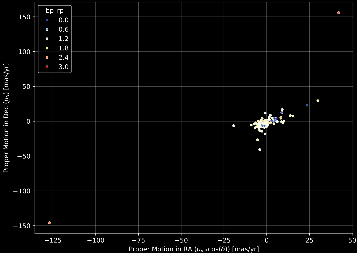
APOGEE DR17 Field: [090+08] Proper Motion Diagram (n= 239)
