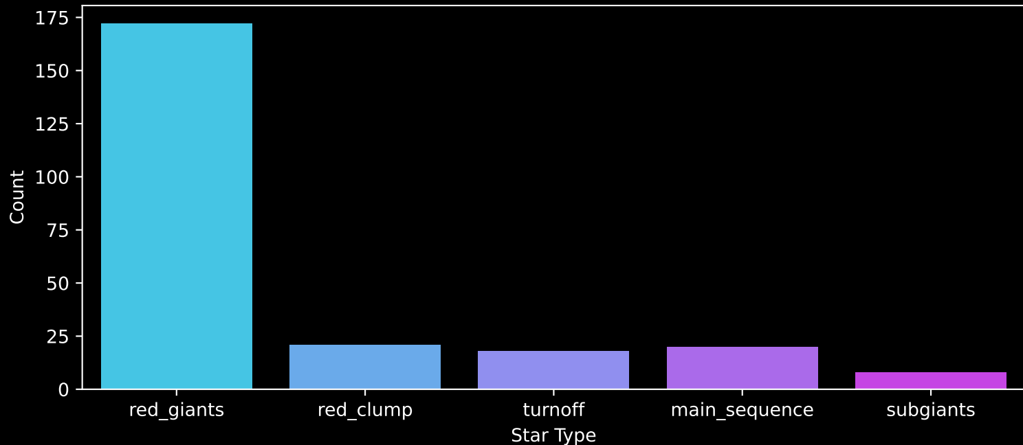
APOGEE DR17 Field: [090+08] Count plot of Star Type
