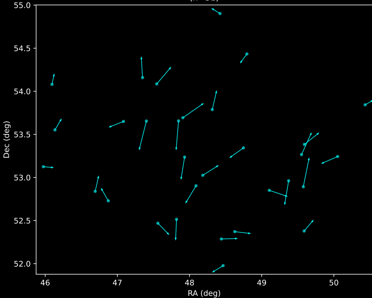
APOGEE DR17 Noise Stream Proper Motion Vectors (n=31)
