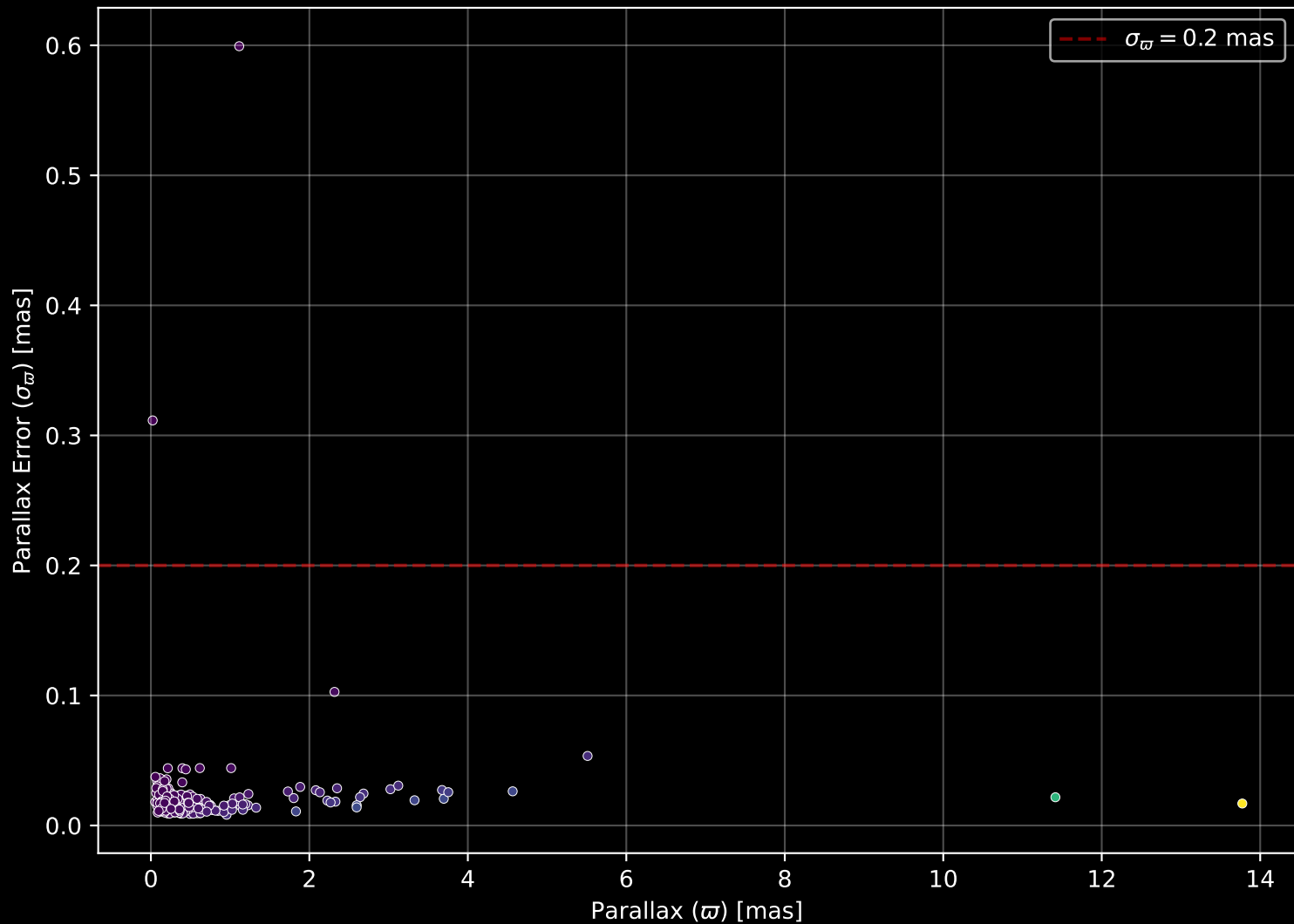
APOGEE DR17 Field: [090+08] Parallax Quality (n= 239)
